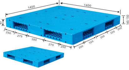
ENL-H1414PSA 140 x 140 x 16 cm
