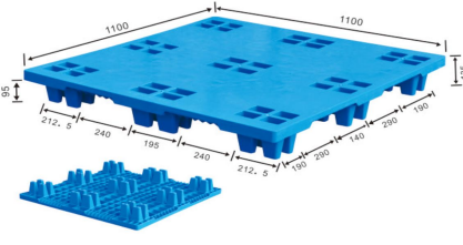
ENL-Y1111PQA 110 x 110 x 13.5 cm
