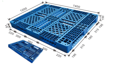
ENL-Y1412WTA 140 x 120 x 15 cm
