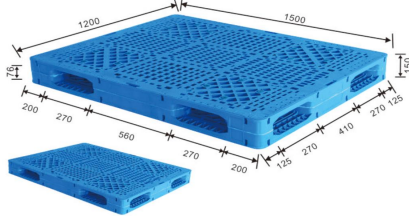
ENL-H1512WSB 150 x 120 x 15 cm
