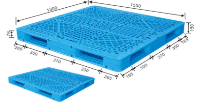
ENL-H1513WSA 150 x 130 x 15 cm
