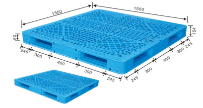
ENL-H1550WSA 155 x 155 x 15.4 cm
