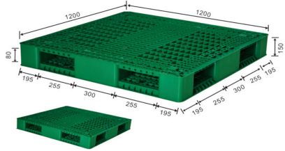
ENL-Y1212WSA 120 x 120 x 15 cm
