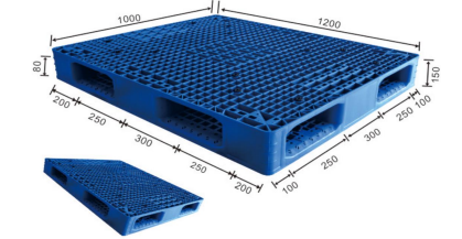
ENL-Y1210WSB 120 x 100 x 15 cm
