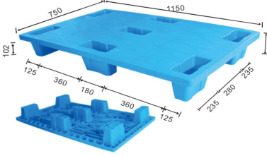
ENL-Y11575PQJ 115 x 75 x 15 cm
