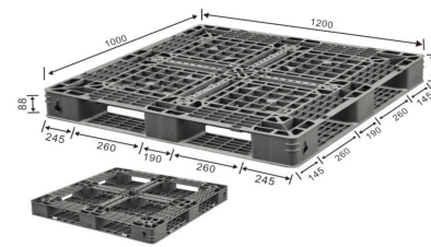
ENL-Y1210WTC 120 x 100 x 12 cm
