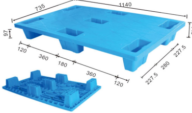
ENL-Y11473PQJ 114 x 73.5 x 14.5 cm
