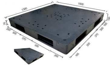
ENL-H1513PSA 150 x 130 x 15 cm
