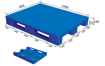
ENL-1208PGC 120 x 80 x 15 cm
