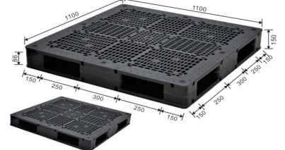
ENL-H1111WSE 110 x 110 x 15 cm
