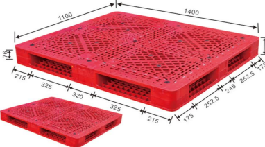
ENL-H1411WSC 140 x 110 x 15 cm
