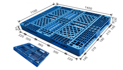
ENL-Y1411WTA 140 x 110 x 15 cm
