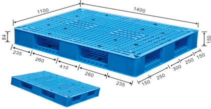
ENL-Y1411WSB 140 x 110 x 15 cm
