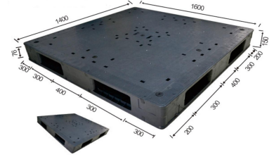
ENL-H1614PSA 160 x 140 x 15 cm
