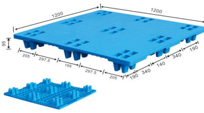
ENL-Y1212PQA 120 x 120 x 13.5 cm
