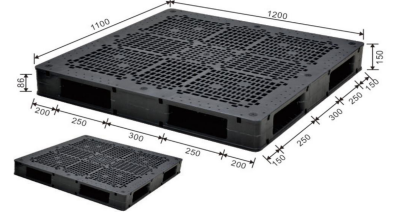
ENL-H1211WSB 120 x 110 x 15 cm
