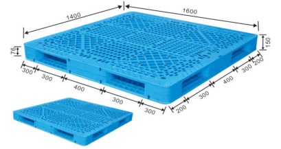
ENL-H1614WSB 160 x 140 x 15 cm
