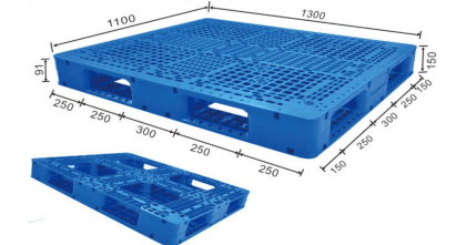
ENL-H1311WTA 130 x 110 x 15 cm
