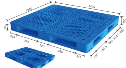
ENL-H1412WTA 140 x 120 x 15 cm
