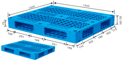
ENL-H1010WSA/B 100 x 100 x 16/15 cm
