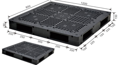
ENL-H1208WSA 120 x 80 x 15 cm
