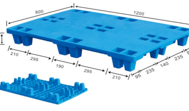
ENL-Y1208PQA 120 x 80 x 13.5 cm
