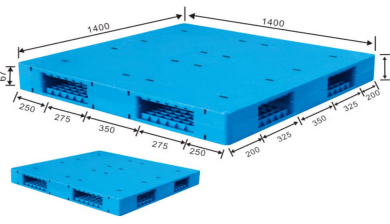
ENL-H1414PSB 140 x 140 x 15 cm
