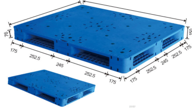
ENL-H1411PSD 140 x 110 x 15 cm
