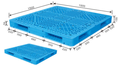
ENL-H1515WSA 150 x 150 x 15 cm
