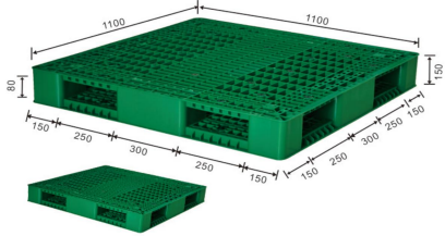
ENL-Y1111WSA 110 x 110 x 15 cm
