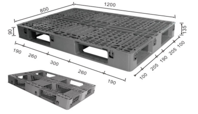
ENL-Y1208WTC 120 x 80 x 13.5 cm
