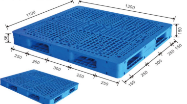
ENL-H1311WSF 130 x 110 x 15 cm
