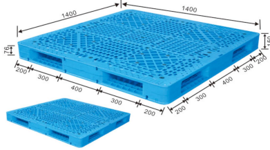
ENL-H1414WSC 140 x 140 x 15 cm
