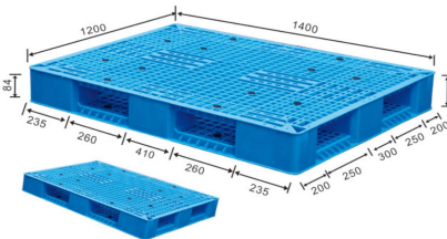
ENL-Y1412WSB 140 x 120 x 15 cm
