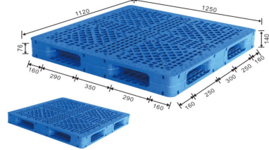
ENL-H125112WSA 125 x 112 x 14 cm
