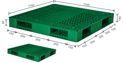
ENL-Y1111WSC 110 x 110 x 15 cm
