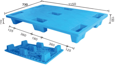
ENL-Y11573PQJ 115 x 73 x 15 cm
