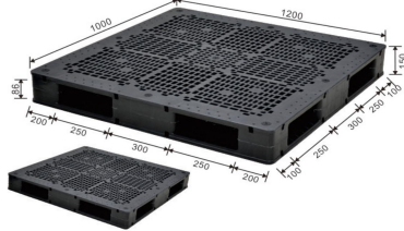
ENL-H1210WSF 120 x 100 x 15 cm
