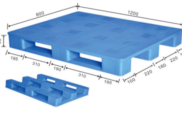
ENL-H1208PHA 120 x 80 x 15 cm
