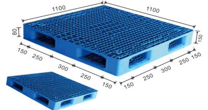
ENL-Y1111WSE 110 x 110 x 15 cm
