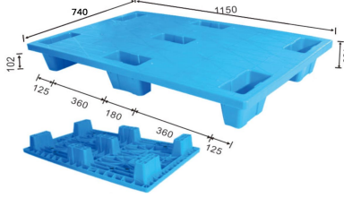
ENL-Y11574PQJ 115 x 74 x 15 cm
