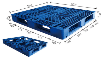
ENL-Y1212WTB 120 x 120 x 15 cm
