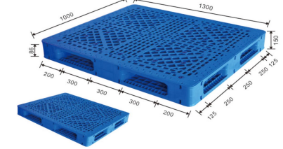
ENL-H1310WSA 130 x 100 x 15 cm
